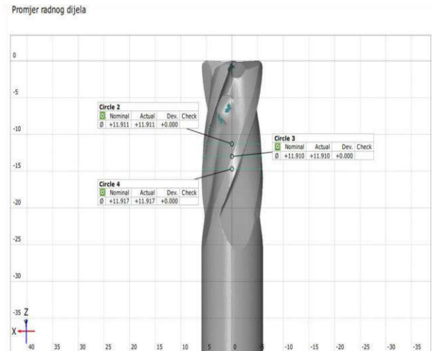
Figure 16. Display of the measurement report page
