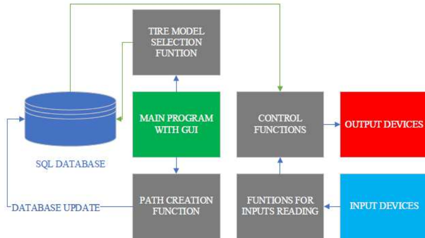
Figure 12. Software architecture
